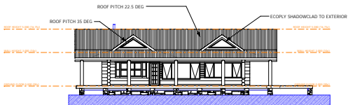
SOUTH ELEVATION
