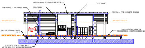
SECTION ELEVATION X-X
